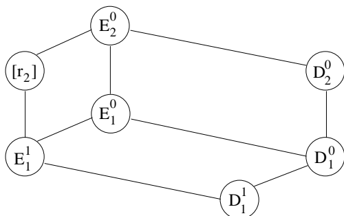
FIG. 7.4. Lattice of all homogeneous relational clones over domain size n = 2 .
