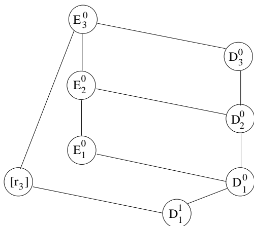
FIG. 7.3. Lattice of all homogeneous relational clones over domain size n = 3 .
