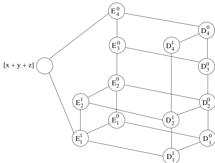
FIG. 7.2. Lattice of all homogeneous relational clones over domain size n = 4 .
