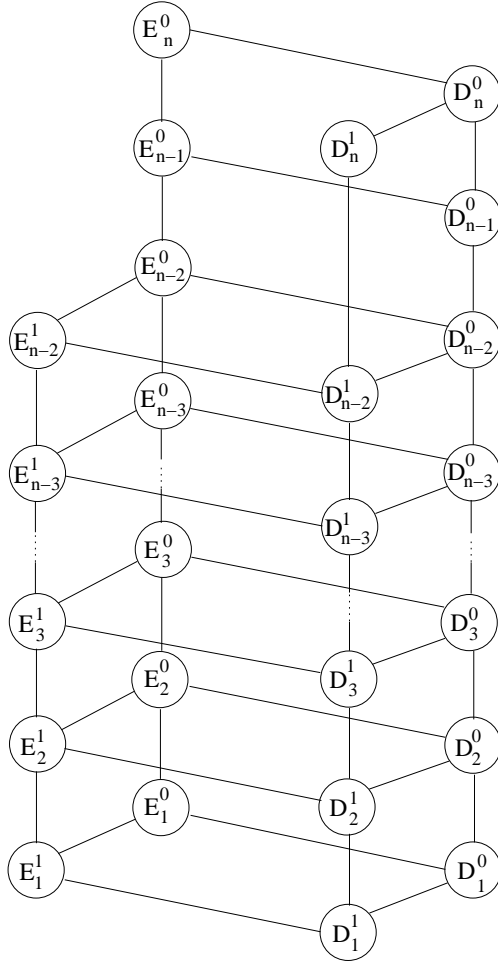
FIG. 7.1. Lattice of all homogeneous relational clones over domain size n \geq 5 .
